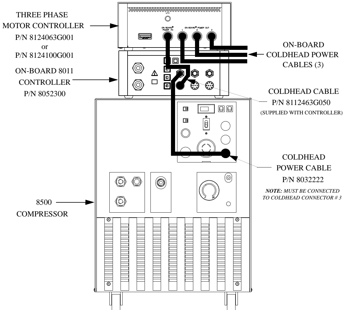
Figure 3-3: 8500 Compressor Cable Connections
