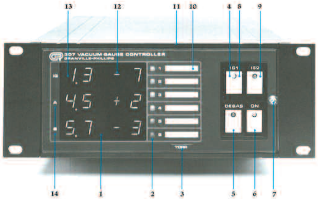
Figure 1. 307 Control Unit
