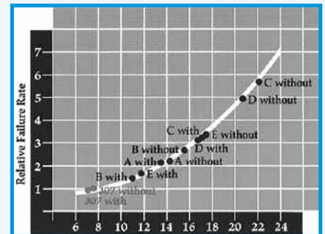
Figure 4: Longer operating life (less probability of component failures) is a benefit of a remote power supply, and cooler operating temperature.
