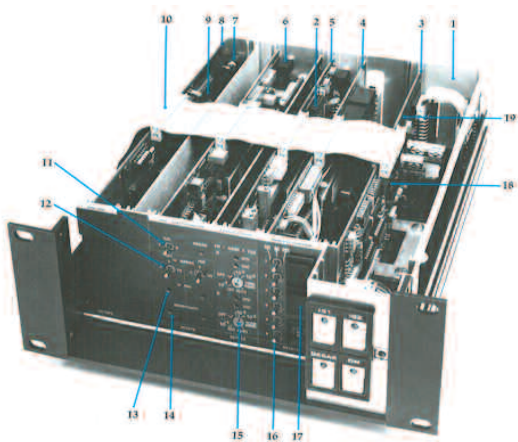
Figure 2. Excellent performance and reliability, intuitive operation and easy, quick maintenance are provided by 307's clean design.
