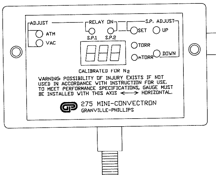
Fig. 3-1 Front Panel Indicators and Adjustments
