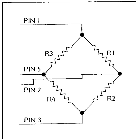
FIG. 2-1 GAUGE TUBE SCHEMATIC
