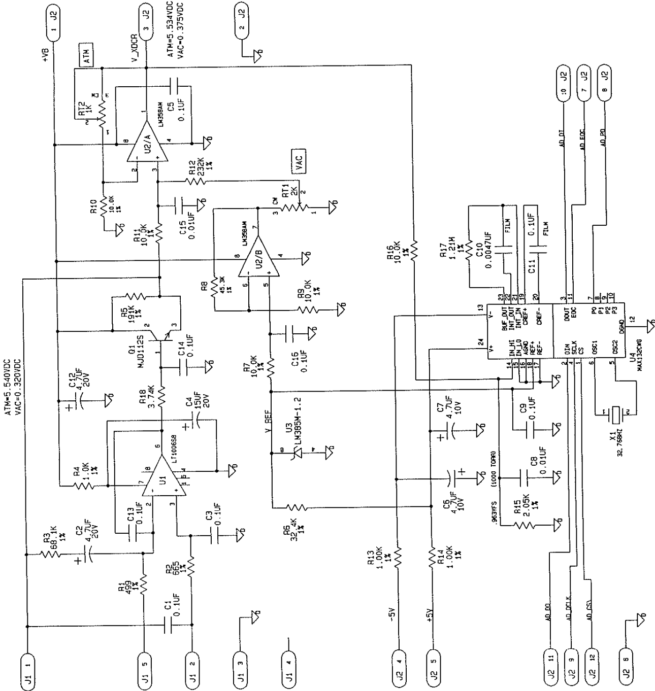
SCHMATIC, 275 DIGITAL DISPLAY BRIDGE
